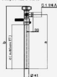
Pumpe F 425 S-41/43
